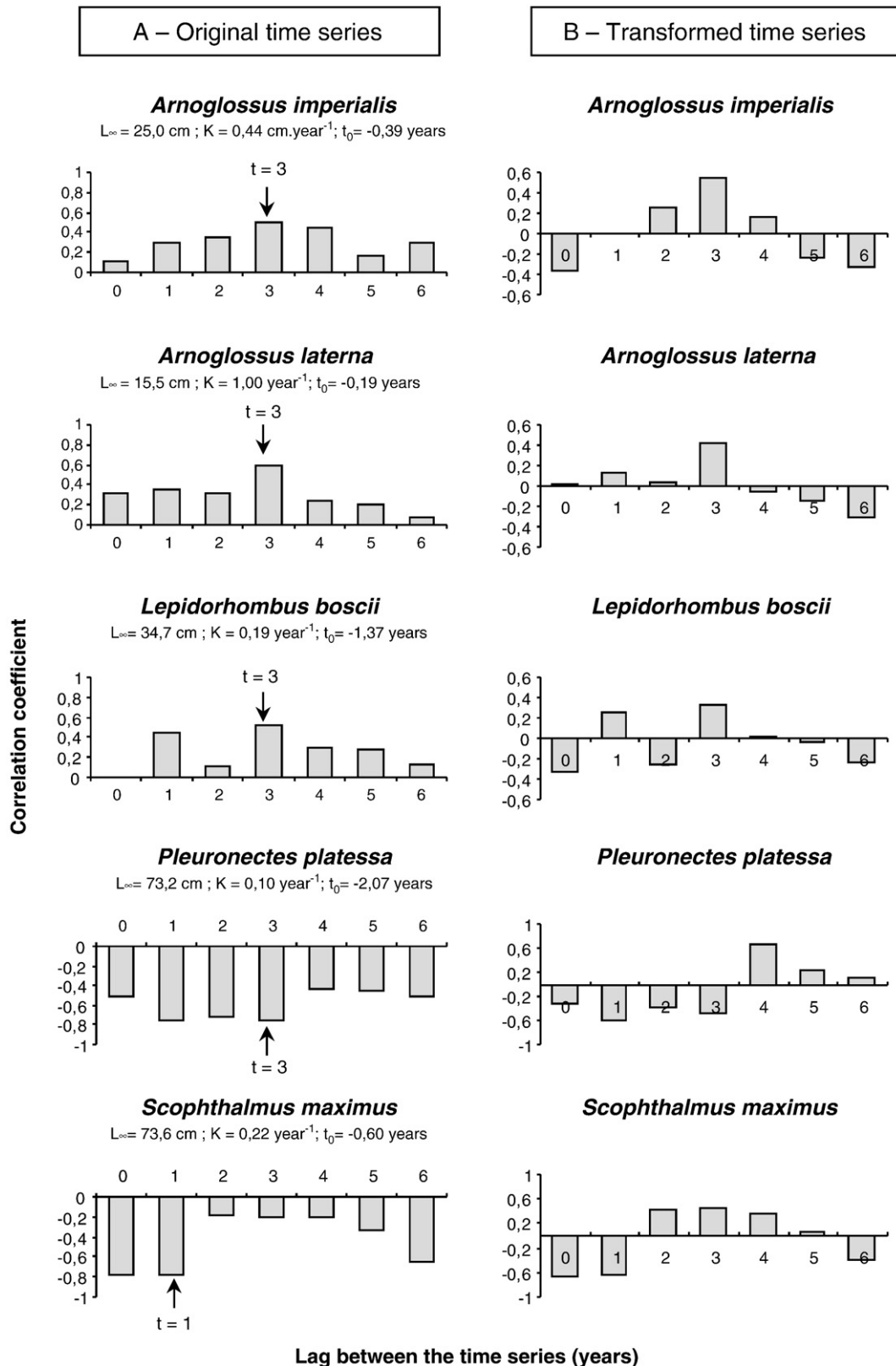
Fig. 5. Coefficients of the linear correlation between mean annual SST and flatfish abundances with a lag from 0 to 6 years between the two time series, using (A) original data and (B) transformed data (after removing trends and autocorrelation). t is the mean age of the populations (expressed in years). Parameters of the Von Bertalanffy growth equation used to calculate this mean age are indicated for each species on part A.
