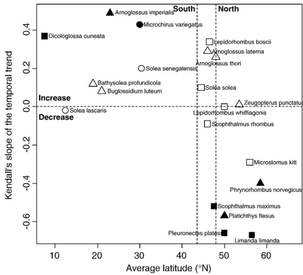
Fig. 3. Relation between the Kendall's slope of the temporal trend in fish densities since 1987 and the mean latitudinal range for the 20 flatfish species caught in the Bay of Biscay. Horizontal dotted line: limit between negative and positive temporal trend; vertical lines: southern and northern limits of the Bay of Biscay. Species are identified with symbols related to their level of exploitation: triangle: not commercial, circle: occasional, square: targeted. Filled symbol corresponds to significant slopes.
