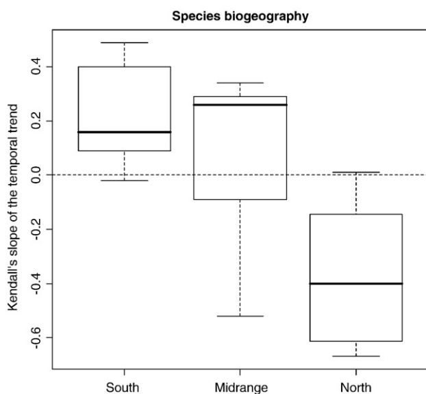
Fig. 4. Boxplots of the distribution of the Kendall's slopes of the temporal trend in fish densities since 1987 for the three groups of flatfish species (southern, centred in the Bay of Biscay, northern).
