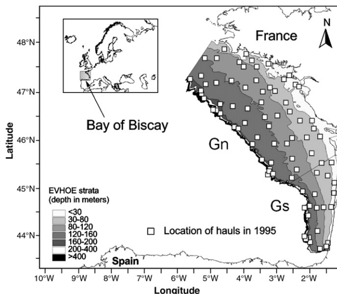
Fig. 1. Map of the Bay of Biscay, with its location in Europe in the upper left corner, showing the area sampled during the 17 groundfish surveys carried out by Ifremer from September to December since 1987, with the sampling design of 1995, given as example. The sampling scheme was stratified according to latitude (Gn, for North, and Gs, for South) and depth.
