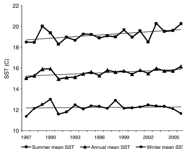
Fig. 2. Time series of the sea surface temperature in the Bay of Biscay for four flatfish species in the Bay of Biscay since 1987.
